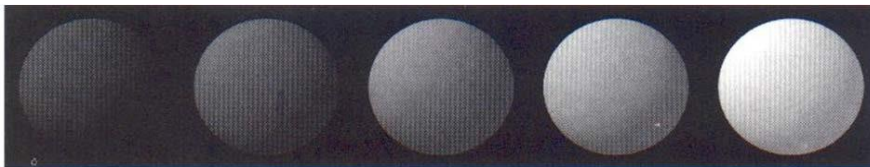
Series of pictures of sphere illuminated by ambient and diffuse reflection model. I_a = I_l = 1.0 , k_d = 0.4 and k_s values (0.0, 0.15, 0.30, 0.45, 0.60).
