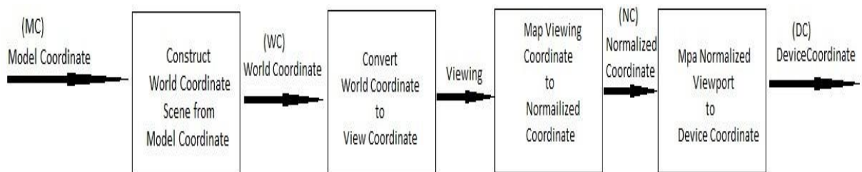
The viewing transformation in several steps, as indicated in above Fig.
