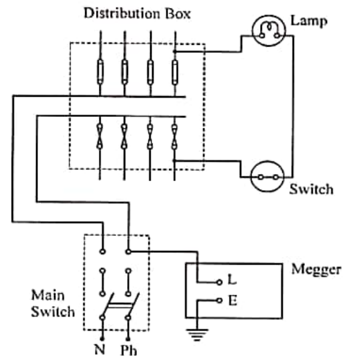
Measurement of insulation resistance to earth
