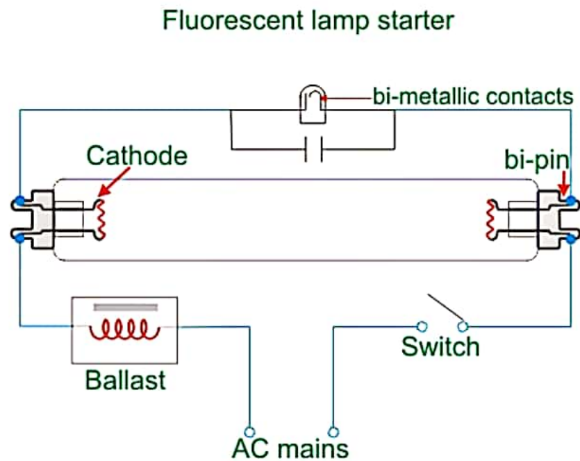
(CIRCUIT DIAGRAM OF CONNECTION OF FLUORESCENT TUBE)
