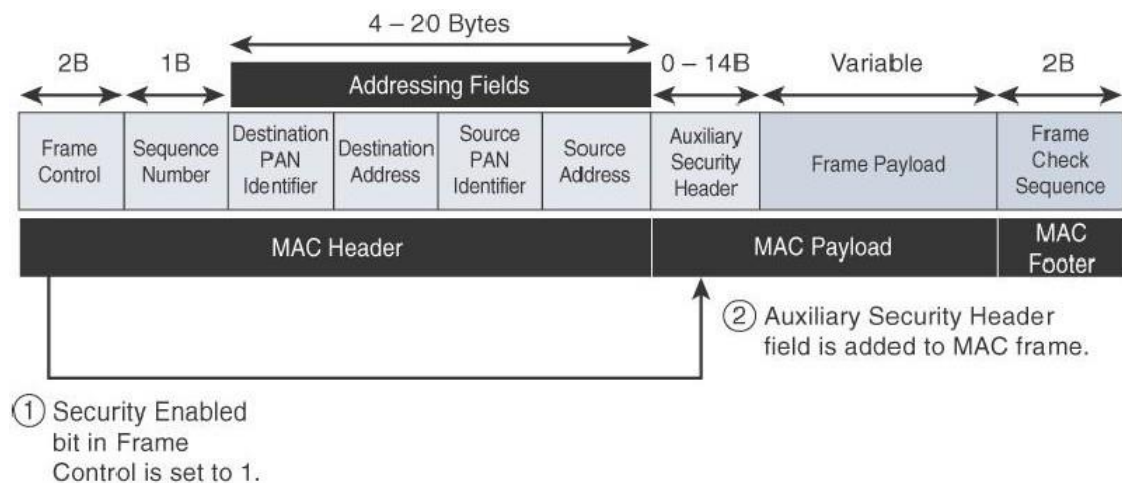
Figure 2.6: Frame format with the Auxiliary Security Header Field for 802.15.4-2006
